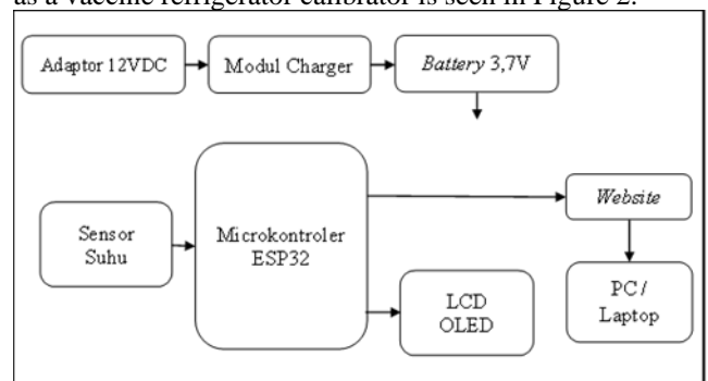
Figure 2. Block Diagram of Data Logger tool as Vaccine refrigerator calibrator
