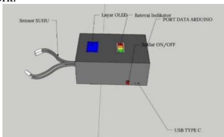
Figure 4. Design of data logger tool design
